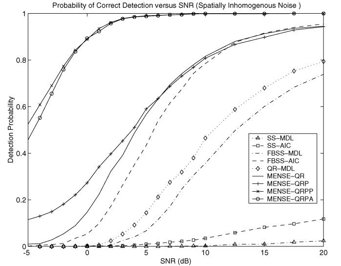
Fig. 11. Probability of correct detection versus the SNR for spatially inhomogeneous noise model for Example 9 ( \nu = 1 , N = 64 , M = 10 , and p = 2 ).
