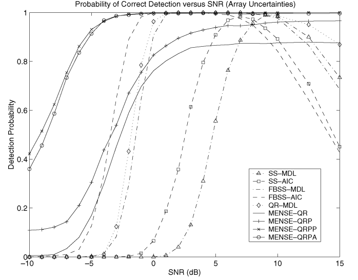
Fig. 10. Probability of correct detection versus the SNR in the presence of array uncertainties for Example 8 ( \sigma_\alpha = 0.1 , \sigma_\phi = 5^\circ , \boldsymbol{\mu} = [1, 0.1, 0.025, 0, \dots, 0]^T , N = 64 , M = 10 , and p = 2 ).
