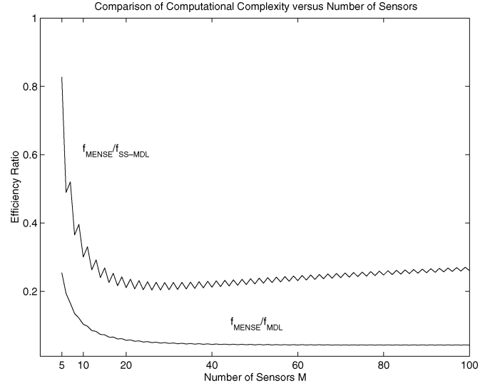
Fig. 1. Relative efficiency ratios between the estimated number of MATLAB flops required by the MENSE algorithm and that needed by the MDL and SS/FBSS-based MDL methods in terms of the number of sensors ( M = 100 and m = \bar{p} = \lfloor M/2 \rfloor ).
