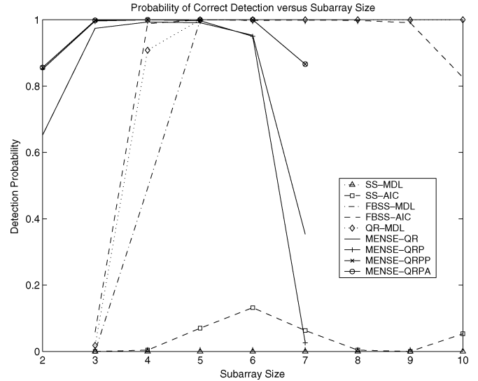
Fig. 6. Probability of correct detection versus the subarray size for Example 4 (SNR = 2.5 dB, N = 64 , M = 10 , and p = 2 ).
