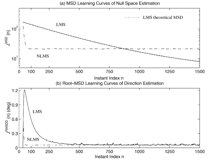
Fig. 6. (a) MSD learning curves of null space estimation and (b) root-MSD learning curves of direction estimation in the case of two coherent signals with constant directions (solid line: LMS ensemble-averaged MSD/root-MSD; dotted line: LMS theoretical MSD; and dashed-dotted line: NLMS ensemble-averaged MSD/root-MSD) for Example 2 ( M = 16 , SNR = 20 dB ( r_s = 1 ), \theta_1 = 10^\circ , \theta_2 = 20^\circ , \mu = 10^{-3} , and \bar{\mu} = 0.1 ).
