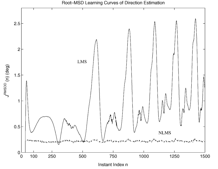
Fig. 8. Root-MSD learning curves of direction estimation for tracking time-varying directions of two coherent signals (solid line: LMS; and dashed-dotted line: NLMS) for Example 3 ( M = 16 , \text{SNR} = 20 dB ( r_s = 1 ), \theta_1(n) = 15^\circ + 0.002^\circ(n-1) , \theta_2(n) = 5^\circ \sin(2\pi(4 \times 10^{-4}n + 2.25 \times 10^{-6}n^2)) , \mu = 2 \times 10^{-3} , and \bar{\mu} = 1 ).
