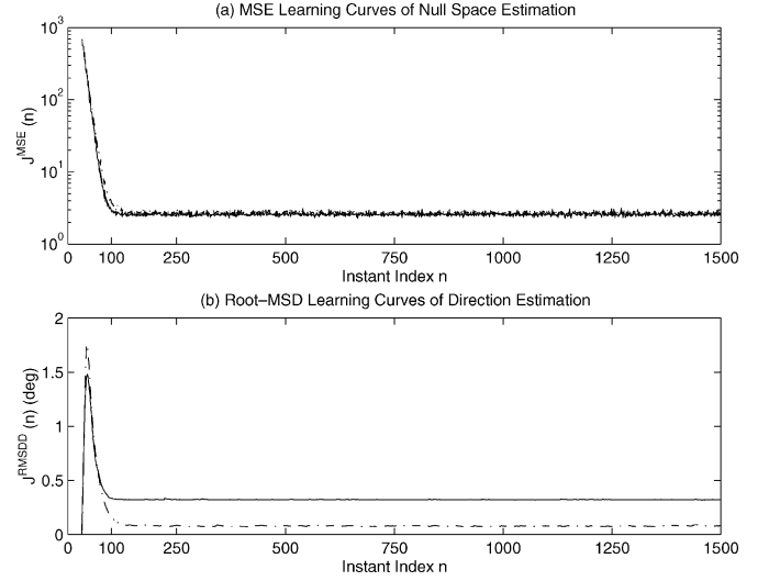
Fig. 11. (a) Ensemble-averaged MSE learning curves of null space estimation and (b) root-MSD learning curves of direction estimation for adaptive estimation of two constant directions (solid line: LMS; and dashed-dotted line: NLMS) for Example 5 ( M = 16 , \text{SNR} = 20 dB, \theta_1 = 10^\circ , \theta_2 = 20^\circ , \bar{p} = 7 , \mu = 10^{-4} , and \bar{\mu} = 0.05 ).
