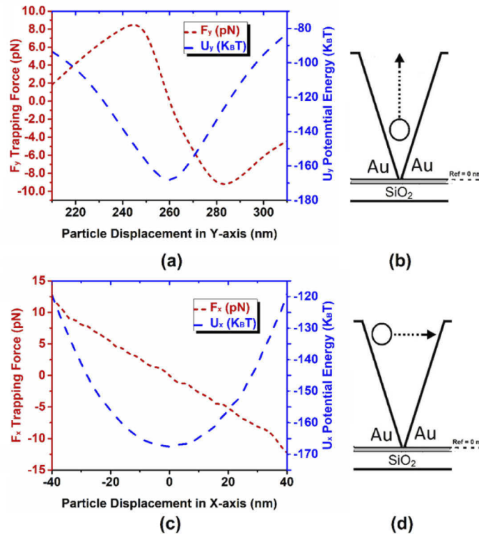
Fig. 6. (a): The vertical trapping force exerted on the 40 nm gold particle and the potential energy distribution as a function particle's displacement locus along the y-axis of the hybrid gold-graphene V-trench optical trap working at 670 nm wavelength. (b): Illustration of the displacement locus of the particle along y-axis. (c) The transverse trapping force exerted on the particle and the potential energy distribution as a function particle's displacement locus along the x-axis of the V-trench optical trap. (d): Illustration of the displacement locus of the particle along x-axis. (Input power intensity is 4 \times 10^9 \text{ W/m}^2 , nanoparticle is immersed in water and Fermi level of graphene monolayer is 0.2 eV.)
