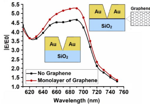
Fig. 3. Comparison of local electric field enhancement ( |E/E_0| ) inside the nano-V-trench between gold (Au) based plasmonic nano-V-trench optical tweezer and gold and graphene based hybrid plasmonic nano-V-trench optical tweezer with monolayer of graphene (thickness 0.335nm). Laser power intensity = 4 \times 10^9 W/m 2 , immersed medium = water (refractive index (n) = 1.33).
