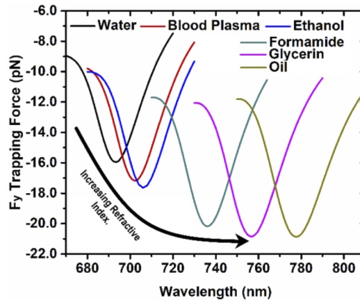
Fig. 5. Vertical trapping force acting on a 40 nm gold particle as a function of incident trapping laser spectra for different surrounding mediums of the optical trap; Water n=1.33 , Blood Plasma n=1.351 , Ethanol n=1.361 , Formamide n=1.428 , Glycerin n=1.473 and Oil n=1.518 . Trapping laser power intensity 4 \times 10^9 \text{ W/m}^2 .
