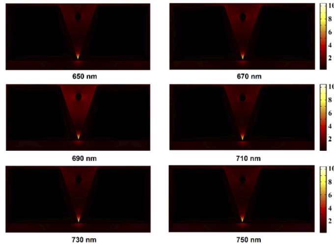
Fig. 2. Electric field distribution color maps inside the nanotrench while 40 nm gold nanoparticle being kept at y = 280 nm position with respect to variation in the wavelength of the incident light beam.
