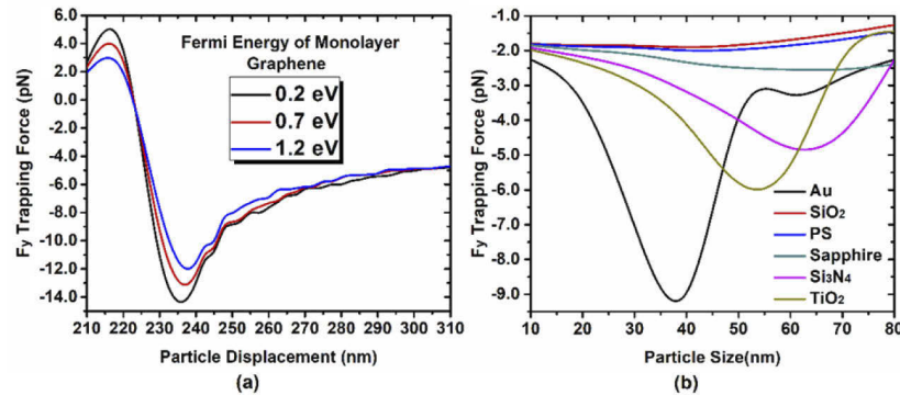
Fig. 4. (a) Vertical trapping force as a function of particle's vertical displacement locus (y-axis) with respect to three different Fermi energy levels of the monolayer graphene (thickness = 0.335 nm). Immersed medium: oil ( n=1.518 ). Laser power intensity = 4 \times 10^9 W/m 2 . Particle = 40 nm gold nanoparticle. (b) Evolution of the vertical trapping force F_y for particles made of different materials (Gold (Au), silica glass (SiO 2 ; n = 1.54 ), polystyrene (PS; n = 1.59 ), Sapphire ( n = 1.77 ), silicon nitride (Si 3 N 4 ; n = 2.2 ) and titanium dioxide (TiO 2 ; n = 2.7 )) as a function of particle size. Particle is kept stationary at 280 nm vertical position while being immersed in water and irradiated by 4 \times 10^9 W/m 2 incident laser power at 670 nm fixed wavelength
