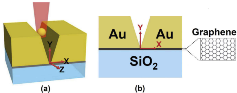
Fig. 1. (a) 3D schematic of the hybrid gold-graphene V-trench plasmonic nanotrap with gold sphere inside the trench being trapped with trapping laser from the top, (b) 2D simulation schematic of the hybrid gold-graphene V-trench plasmonic nanotrap.
