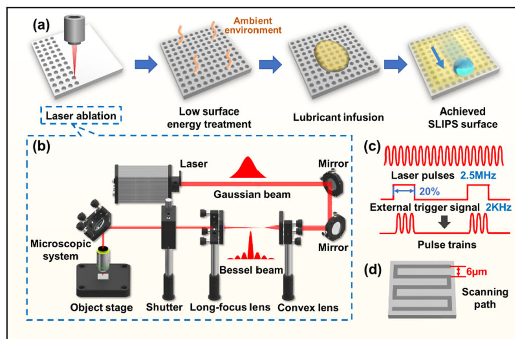
Figure 1. Femtosecond laser fabrication of porous microstructures on the NiTi alloy substrates: (a) Fabrication of the SLIPS on the NiTi alloy. (b) Optical path of the femtosecond laser fabrication system. (c) Illustration of externally triggered laser pulse trains. (d) Scanning path controlled by the object stage.
