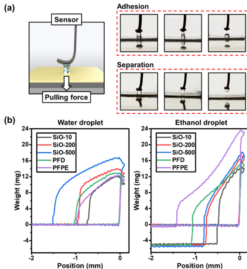
Figure 3. Droplet adhesion force tested with water and ethanol: (a) Adhesion and separation occurred between the droplet and the surface. (b) Droplet adhesion of water and ethanol on the prepared samples tested using high-precision sensors.
