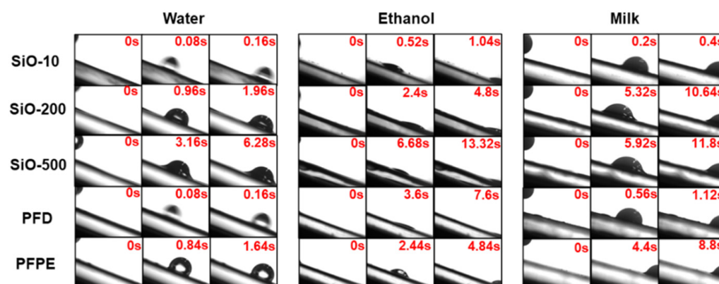
Figure 4. Sliding process and time spent for three liquids (water, ethanol, and milk) on the lubricant-infused samples.
