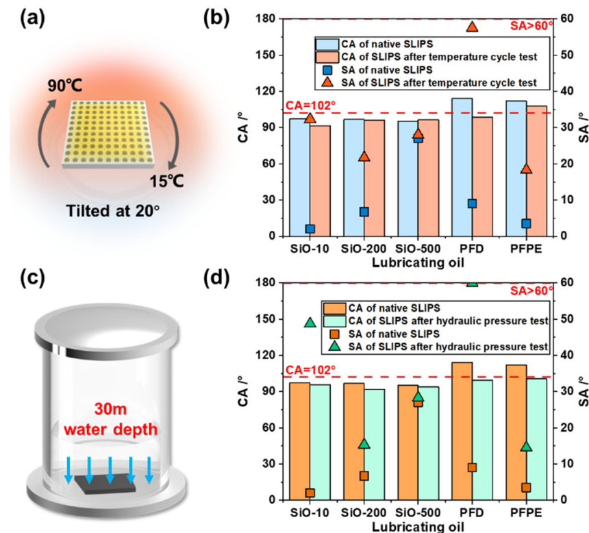
Figure 5. Durability test implemented on the SLIPS samples: (a–d) CA and SA of five lubricant-infused surfaces before and after the temperature cycle test and the hydraulic pressure test. The CA and SA of the NiTi alloy after 7 days are marked by the red lines.
