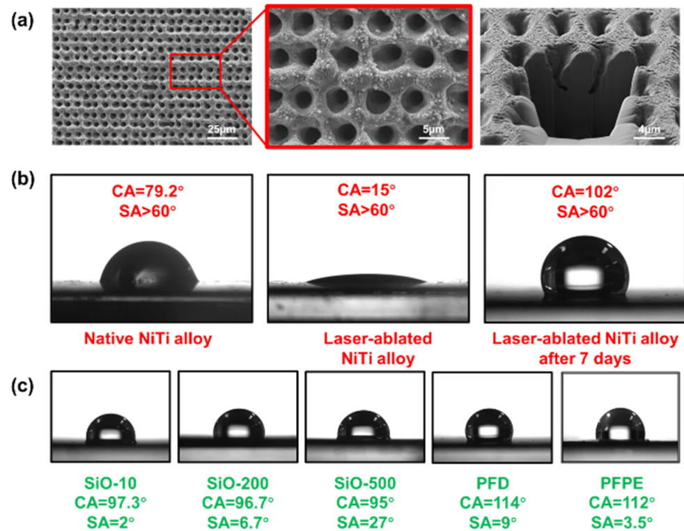
Figure 2. Microstructure of the NiTi alloy surface and its water-repellent properties: (a) Top view and cross-sectional view of the structure taken by scanning electron microscope. (b) Wettability of the native NiTi alloy samples after laser ablation and after being placed in air for 7 days. (c) Wettability of the SLIPSs prepared using SiO-10, SiO-200, SiO-500, PFD, and PFPE.
