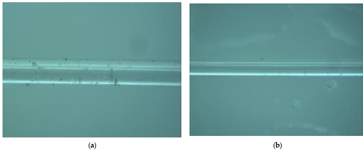
Figure 10. Optical fiber sensor before and after the etching: (a) Optical fiber before etching 125 \mu\text{m} ; (b) Optical fiber after etching 60 \mu\text{m} .
