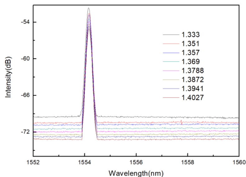
Figure 19. Reflection spectra of corroded FBG sensor with different refractive index.
